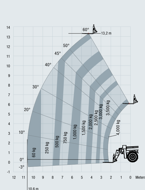
STH1840 – OUTRIGGERS UP
